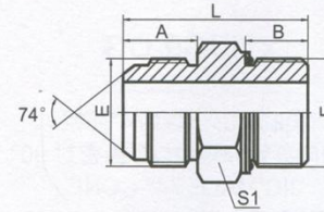
1JG 美制JIC外螺纹74°外锥 / 英管外螺纹O形圈 JIC MALE 74° CONE / BSP MALE O-RING
